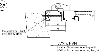
CORNER ASSEMBLY (Wall embedded counterframe)
