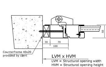
HALLWAY ASSEMBLY (with external wall counterframe)
